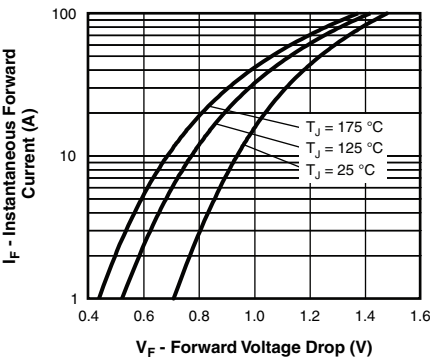
Fig. 1 - Typical Forward Voltage Drop Characteristics
