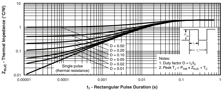
Fig. 4 - Maximum Thermal Impedance Z_{thJC} Characteristics
