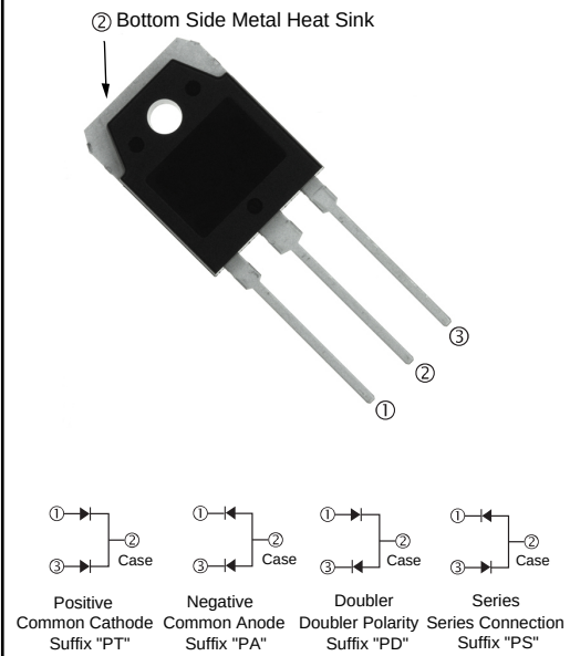
TO-3PN
